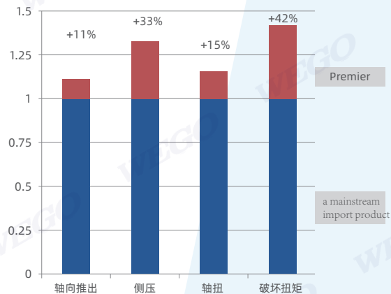
Comparison of mechanical properties of Premier VS a mainstream import product
